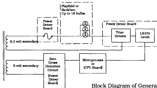
Block Diagram of General Illumination Circuit
