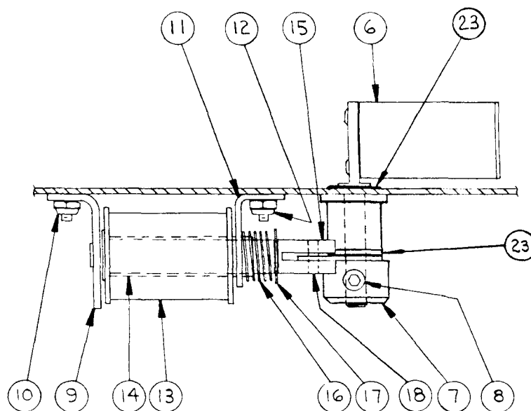
DETAIL VIEW (SHOWN IN ACTUATED POSITION)
