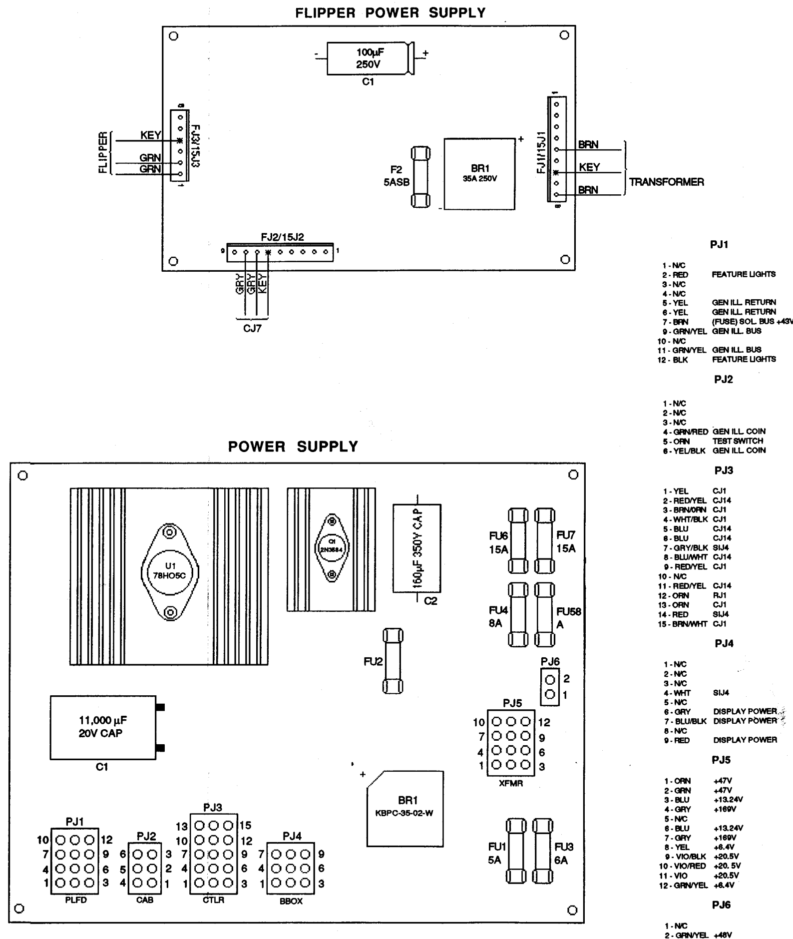
Flipper Power Supply (C-9939-554) Assembly Drawing
