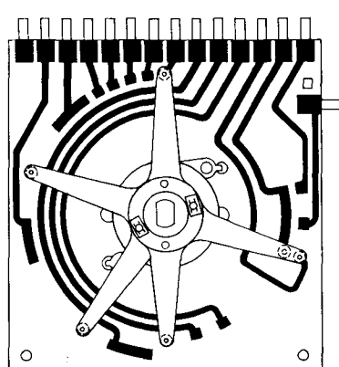
BALL COUNT UNIT PLATE 347-2513 FINGER 308-2505
