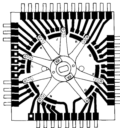
PLAYER CONTROL NO. 2 PLATE NO. 2 393-2509 FINGER NO. 2 393-2510
