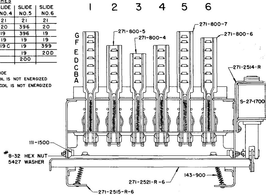
COMPLETE SLIDE TYPE RELAY 393-271-2520-R-6
