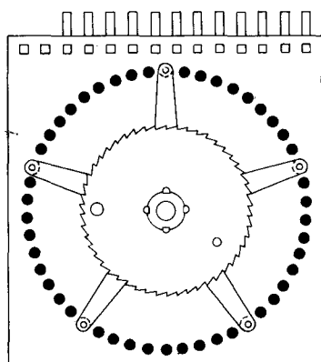
FLASH-O-MATIC PLATE 417-2508 FINGER 176-2502
