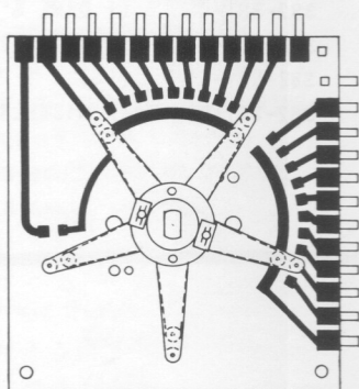
BALL COUNT UNIT PLATE ASS'Y. 455-2510-A-P.C. FINGER ASS'Y. 464-2507
