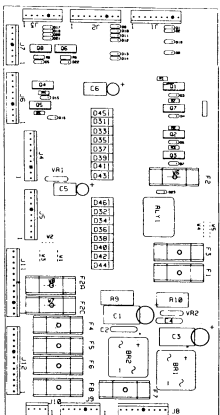
Aux Power Driver Unit Board m1012207
