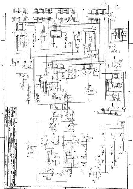
Audio Board (D-12338) Schematic
