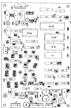
Audio Board PN D-1232-587
