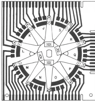
PLAYER CONTROL UNIT PLATE 469-502 FINGER ASS'Y. 456-2507
