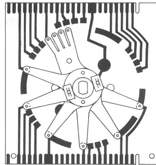
COIN UNIT PLATE 469-500 FINGER ASS'Y. 469-2501
