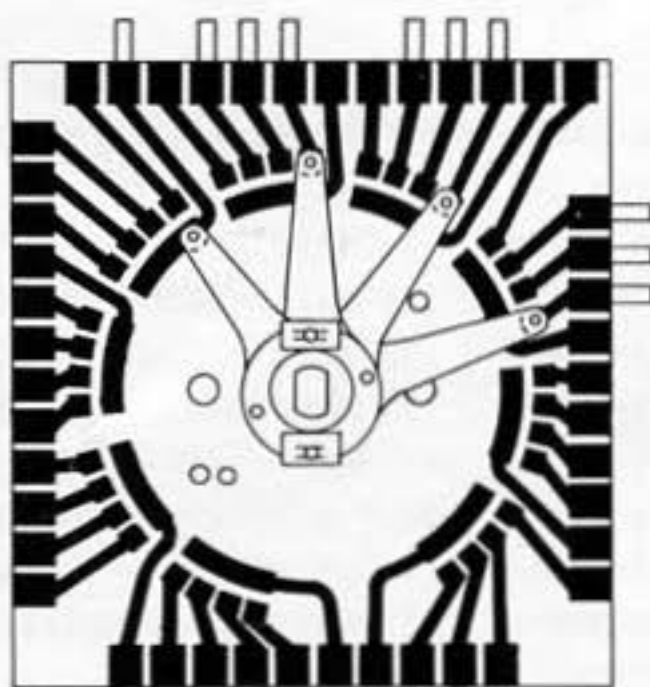
HOLE UNIT PLATE ASS'Y. 460-2506 FINGER ASS'Y. 460-2505
