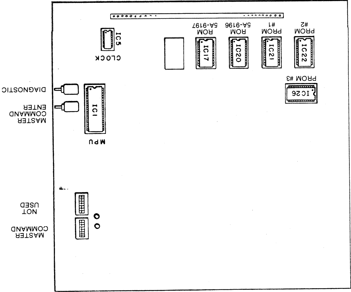
Figure 3. Location of Socketed Components and Switches on CPU Board
