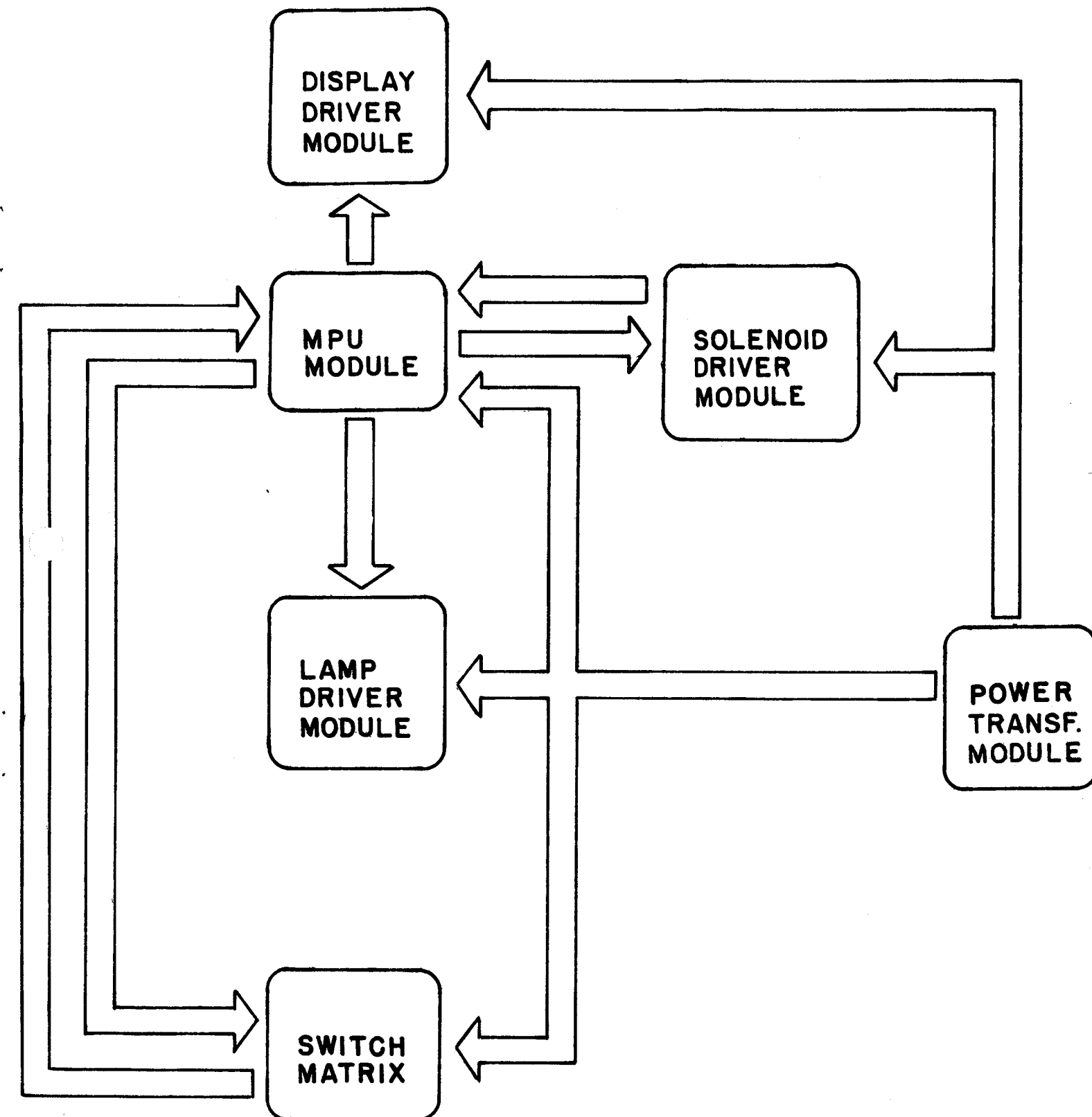
BLOCK DIAGRAM
