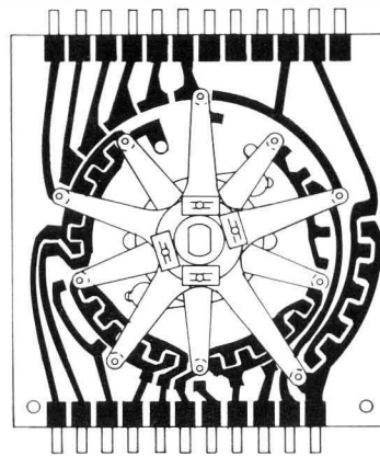
BALL COUNT UNIT PLATE ASS'Y. 455-2510 FINGER ASS'Y. 455-2513
