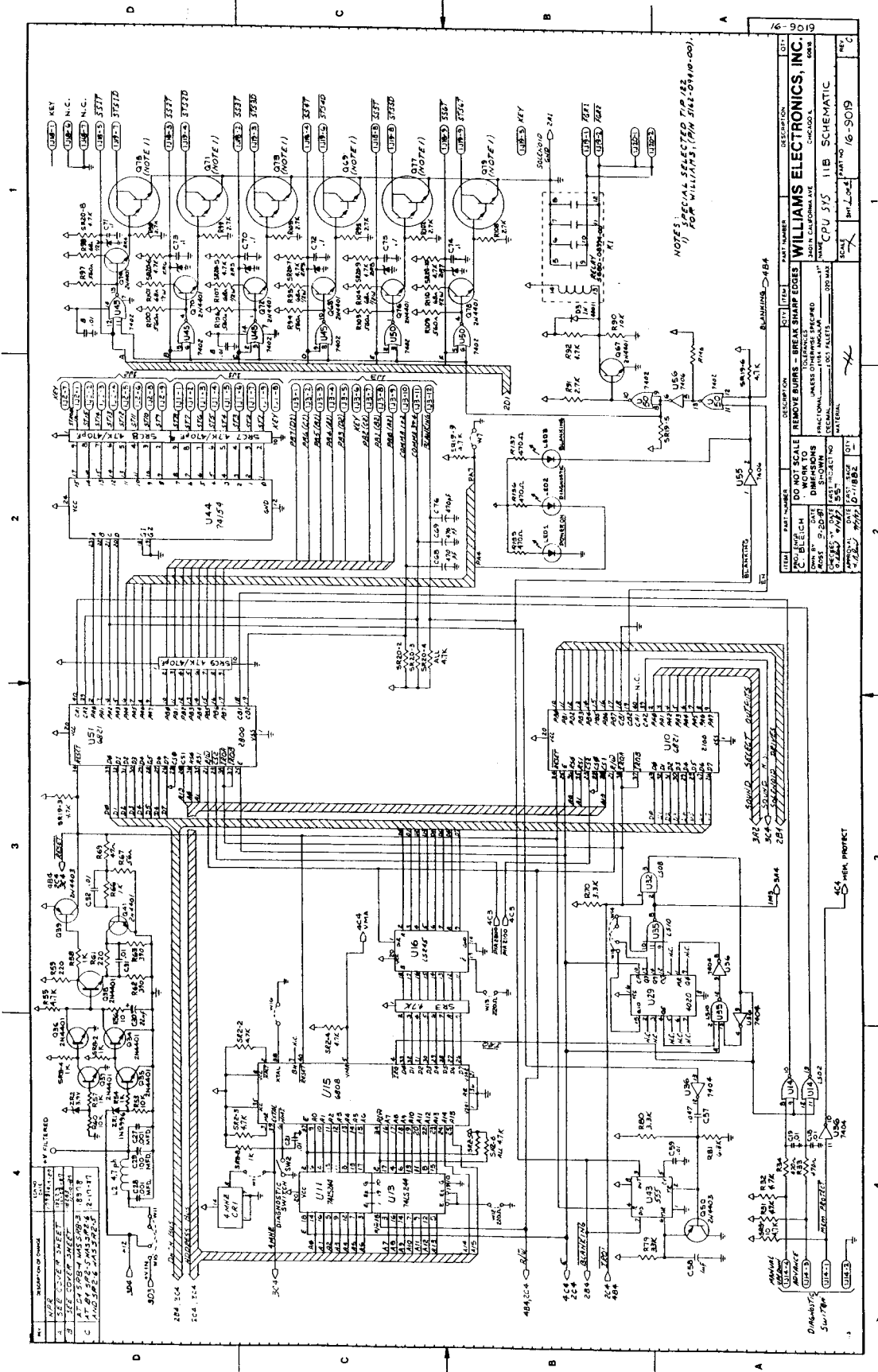
System 11B CPU Schematic (16-9019, Sheet 1 of 4)
