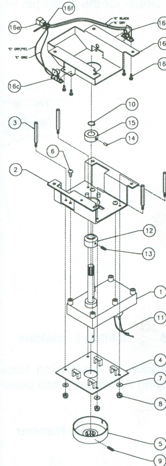
A-19782 MAGIC TRUNK MOTOR ASSY.
