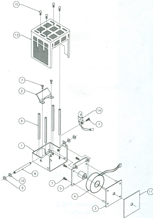
A-19778 MAGIC TRUNK ASSEMBLY
