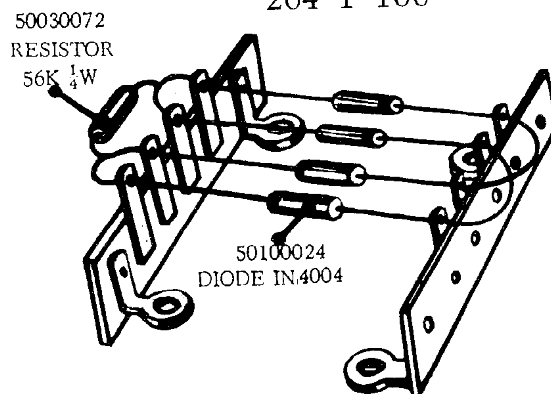
RECTIFIER BRIDGE ASS'Y. 264-1-109
