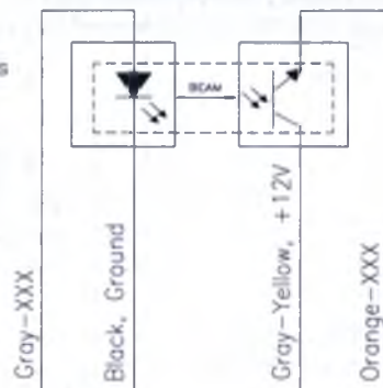
component side
