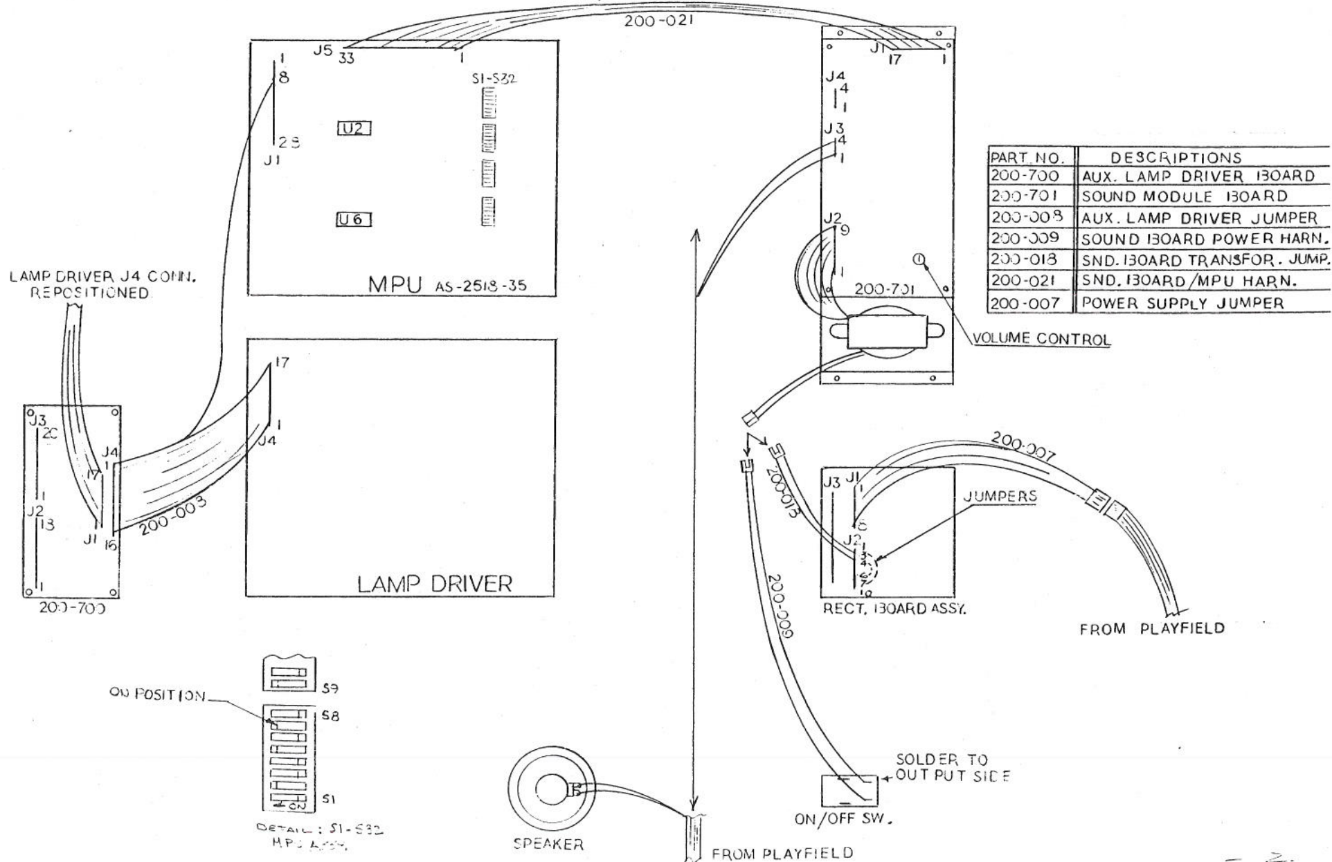
FIGURE 1. ELECTRONIC BOARD/CABLE LAYOUT
