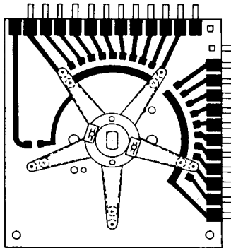
00-90 UNIT PLATE ASS'Y. 344-2515-L FINGER ASS'Y. 344-2506
