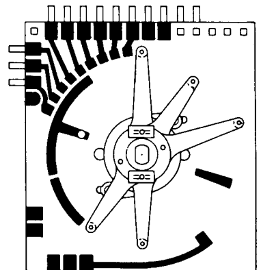
BONUS UNIT PLATE 373-2510-E FINGER 431-2501
