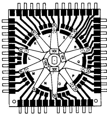
PLAYER CONTROL UNIT PLATE ASS'Y. 456-2506 FINGER ASS'Y. 456-2507
