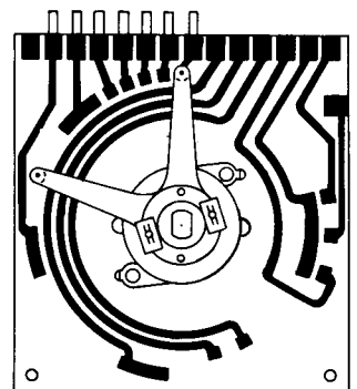
BALL COUNT UNIT PLATE ASS'Y. 347-2513-D FINGER ASS'Y. 465-2501
