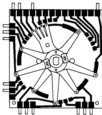
COIN UNIT PLATE ASS'Y. 456-2503 FINGER ASS'Y. 456-2502
