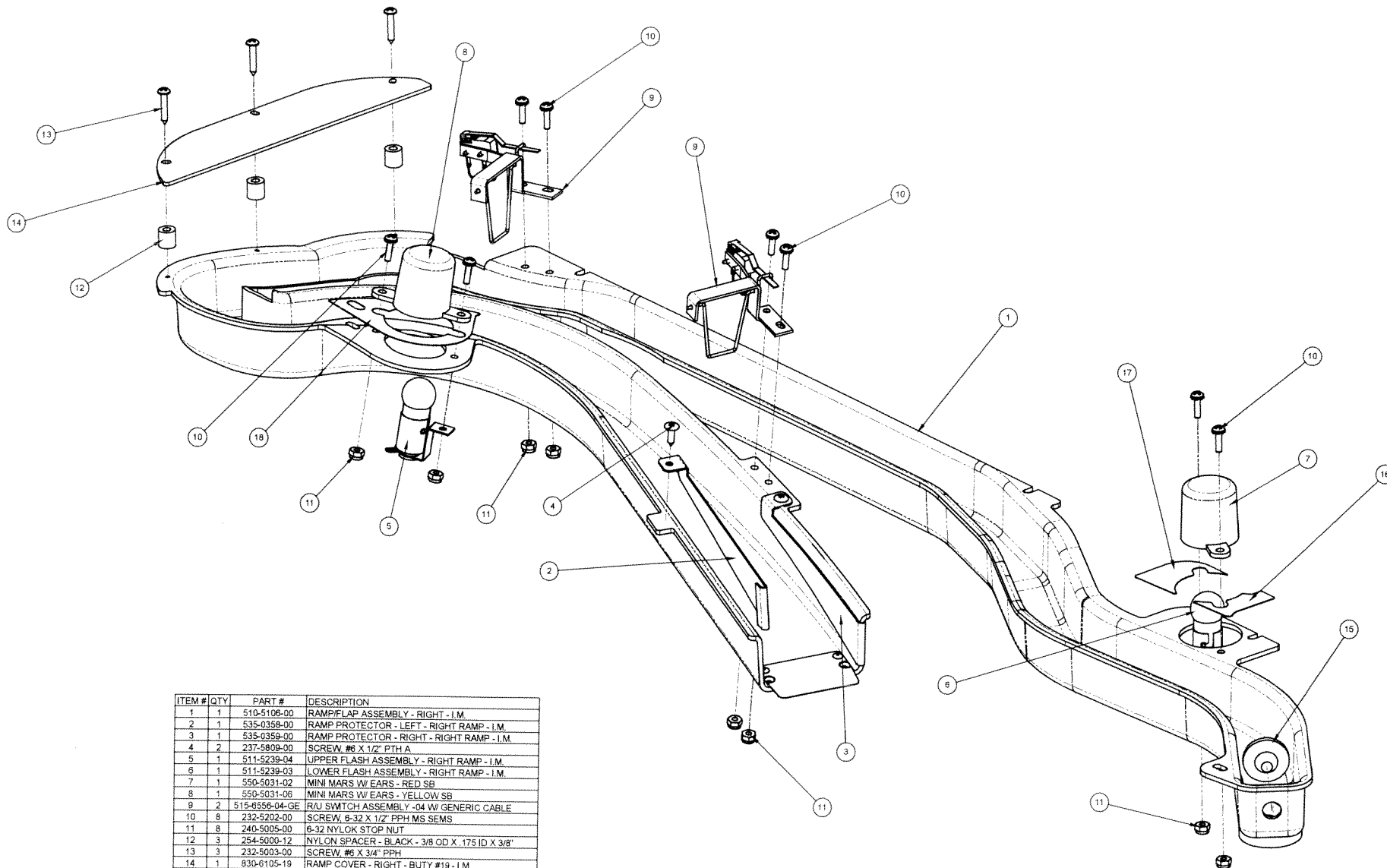
RIGHT RAMP ASSEMBLY - I.M.
