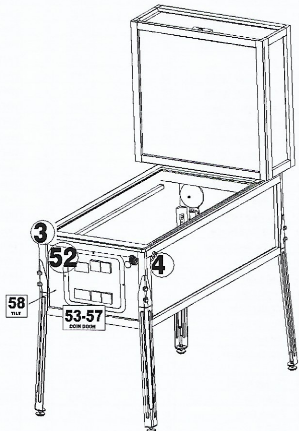
Figure 3.3.3. Cabinet switch locations.
