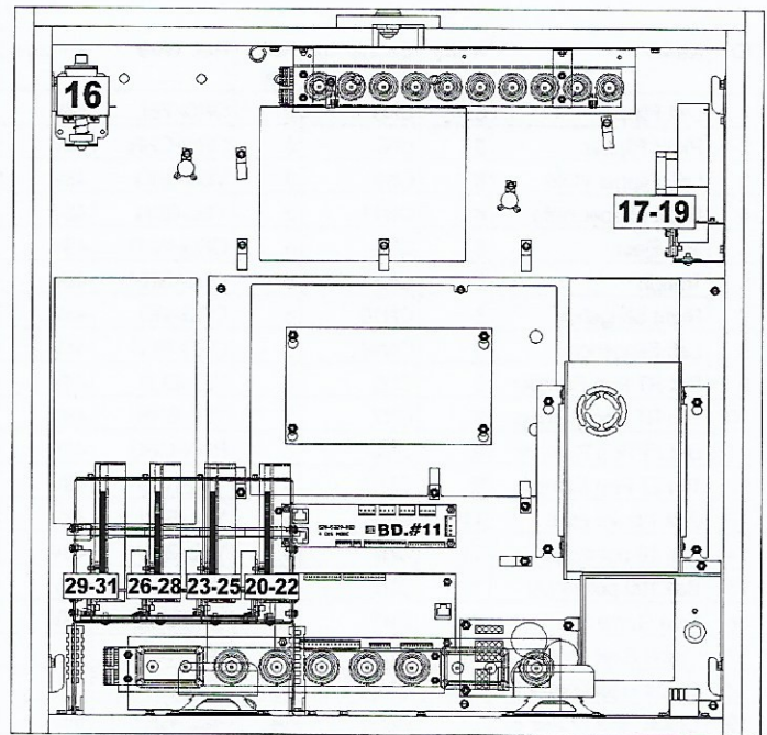
Figure 3.2.2. Backbox driver locations.
