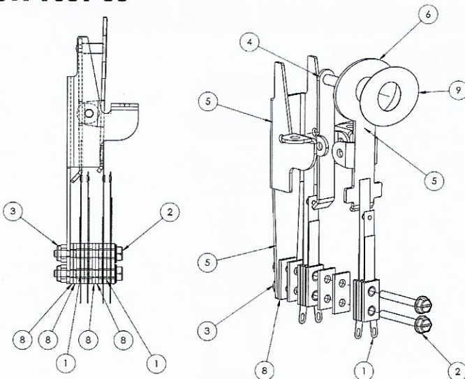
Figure 5.19.3. Trough Coil Assy 500-7286-00 bill of materials.
