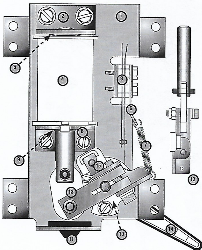
Figure 5.16.1. Flipper Assy, Left Classic 500-6543-84-ND diagram.
