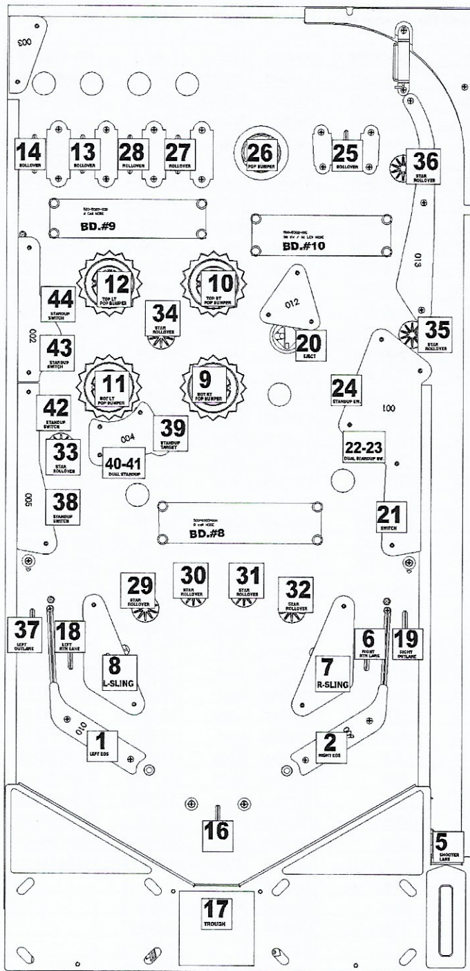
Figure 3.3.1. Switch locations, playfield top view.
