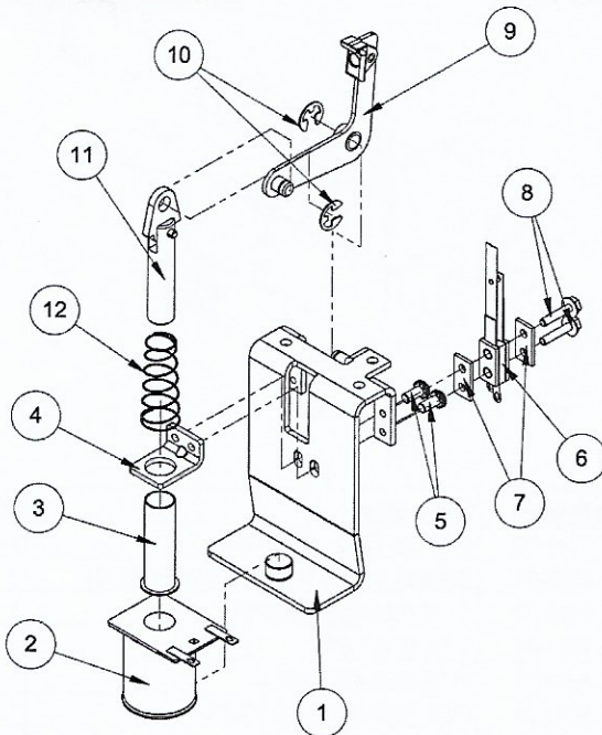
Figure 5.24.1. Sling shot core assembly explosion.
