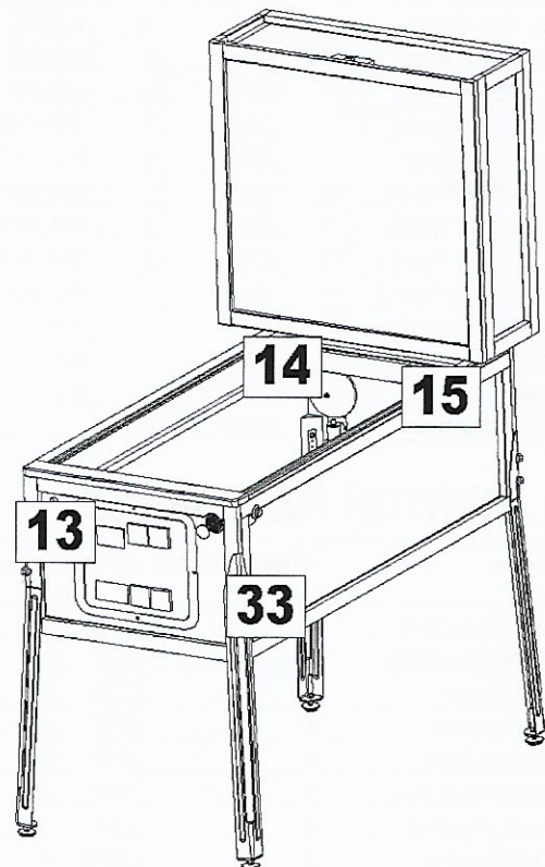
Figure 3.2.3. Cabinet driver locations.
