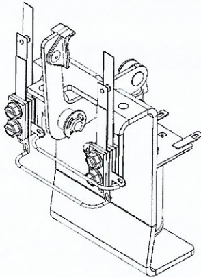
Figure 5.24.4. 500-9920-01-D7 sling shot assembly.
