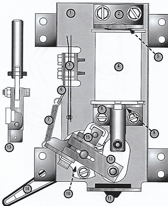
Figure 5.15.4. Flipper Assy, Right Classic 500-6543-85-ND diagram.
