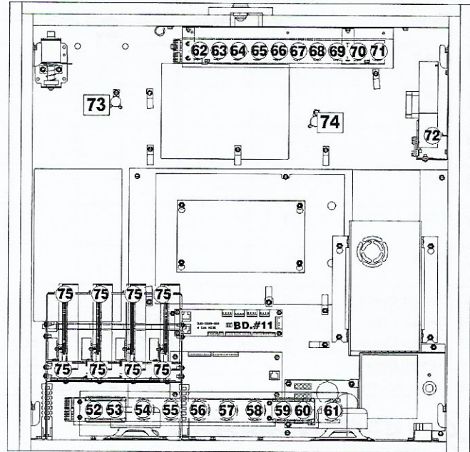
Figure 3.4.2. Backbox light locations.
