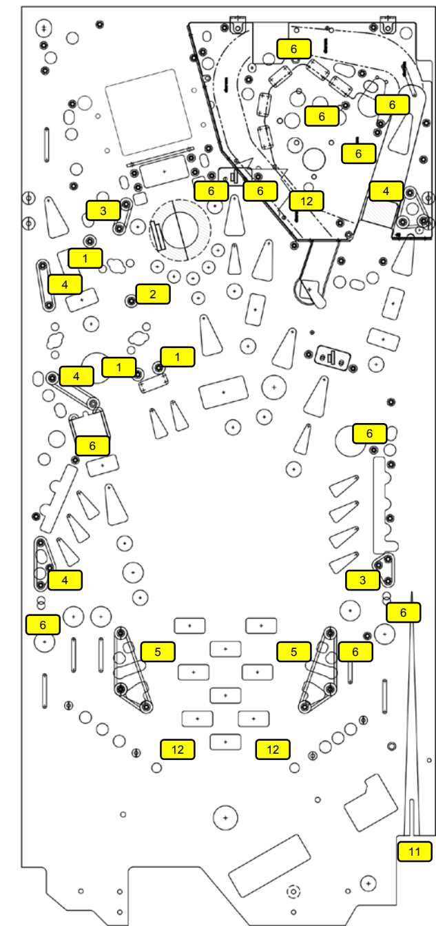
Figure 5.1.1. Rubber o-ring part locations.
