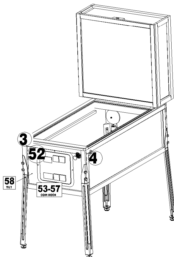
Figure 3.3.3. Cabinet switch locations.
