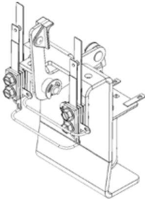
Figure 5.24.2. 500-9920-01-D7 sling shot assembly.
