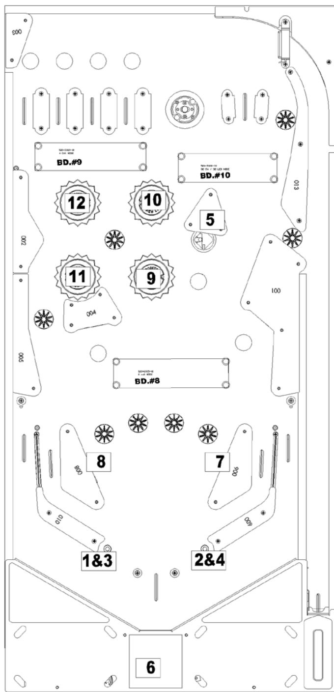
Figure 3.2.1. Playfield top component view.
