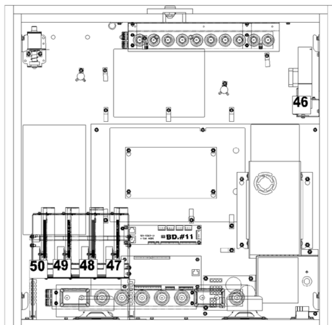
Figure 3.3.2. Backbox switch locations.
