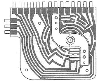
COUNTER SWITCH PLATE 500-2520 FINGER 500-2519
