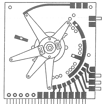
SHOT COUNT CONTACT PLATE PLATE 373-2510-C FINGER 379-2529
