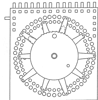
FLASHING BULLS HEAD TARGETS PLATE 404-2523 FINGER 404-2522
