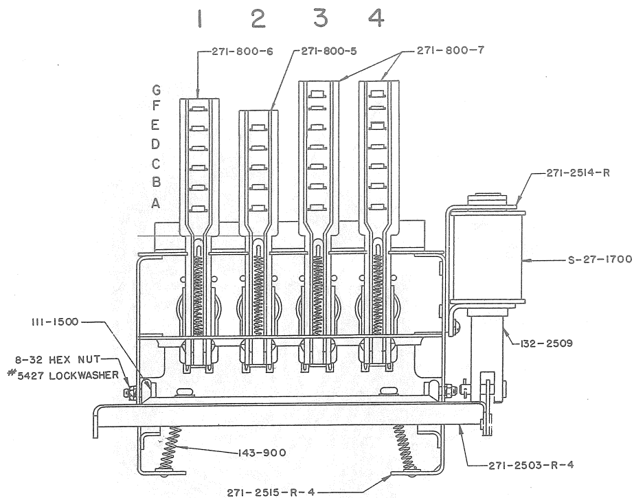
COMPLETE SLIDE TYPE RELAY 404-271-2520-R-4
