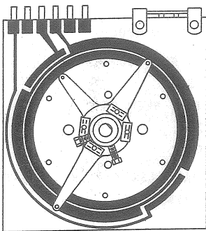
MISS SHOT PRINTED CIRCUIT PLATE 392-2504-A FINGER 404-2520
