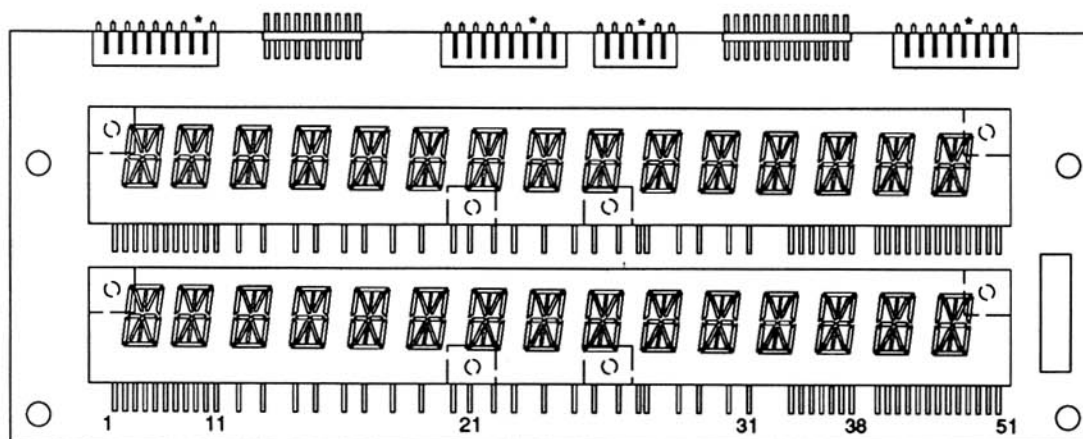
16-Character Display Glass p/n 5670-12308-00
