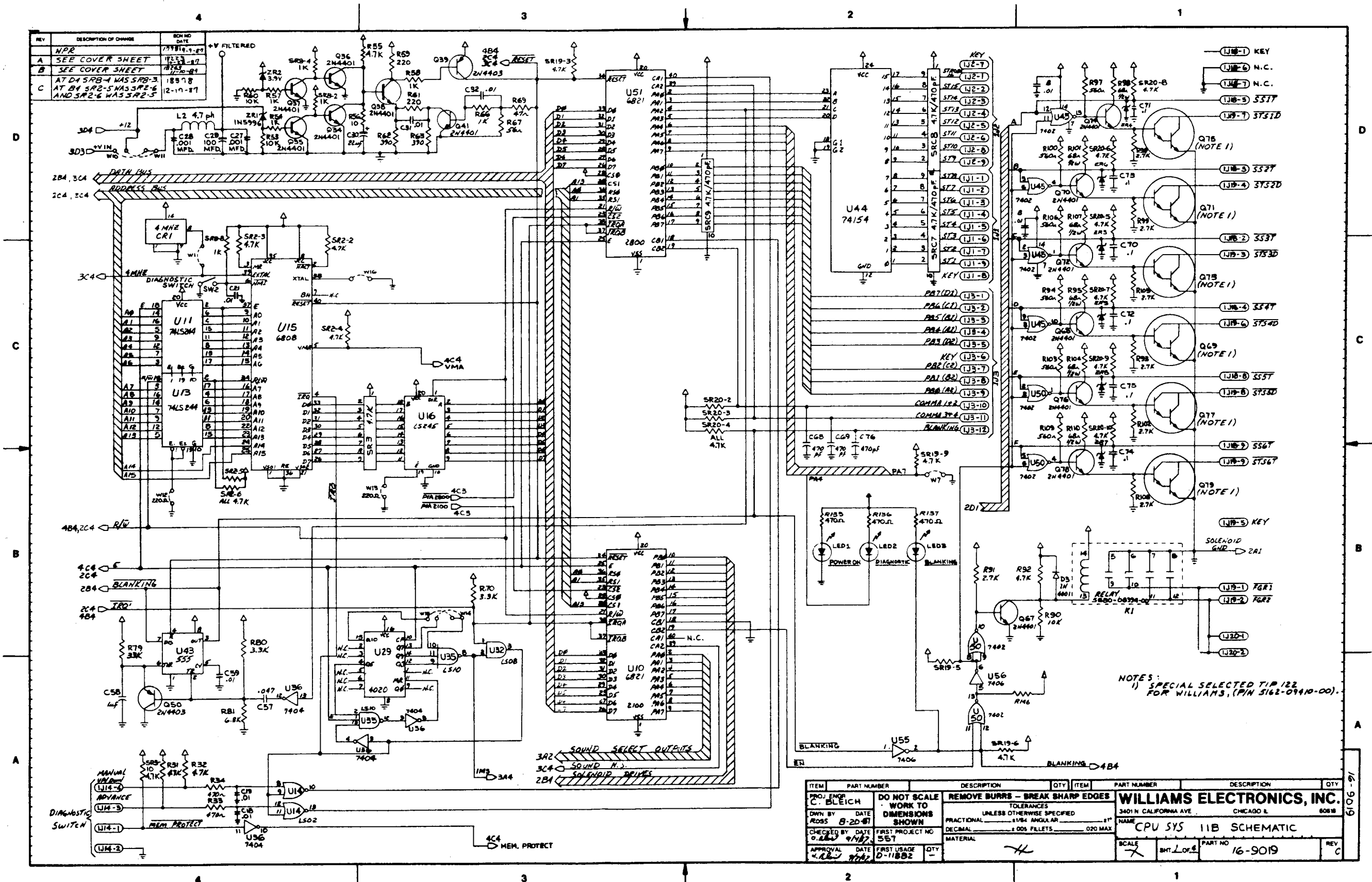
System 11B CPU Schematic (16-9019, Sheet 1 of 4)
