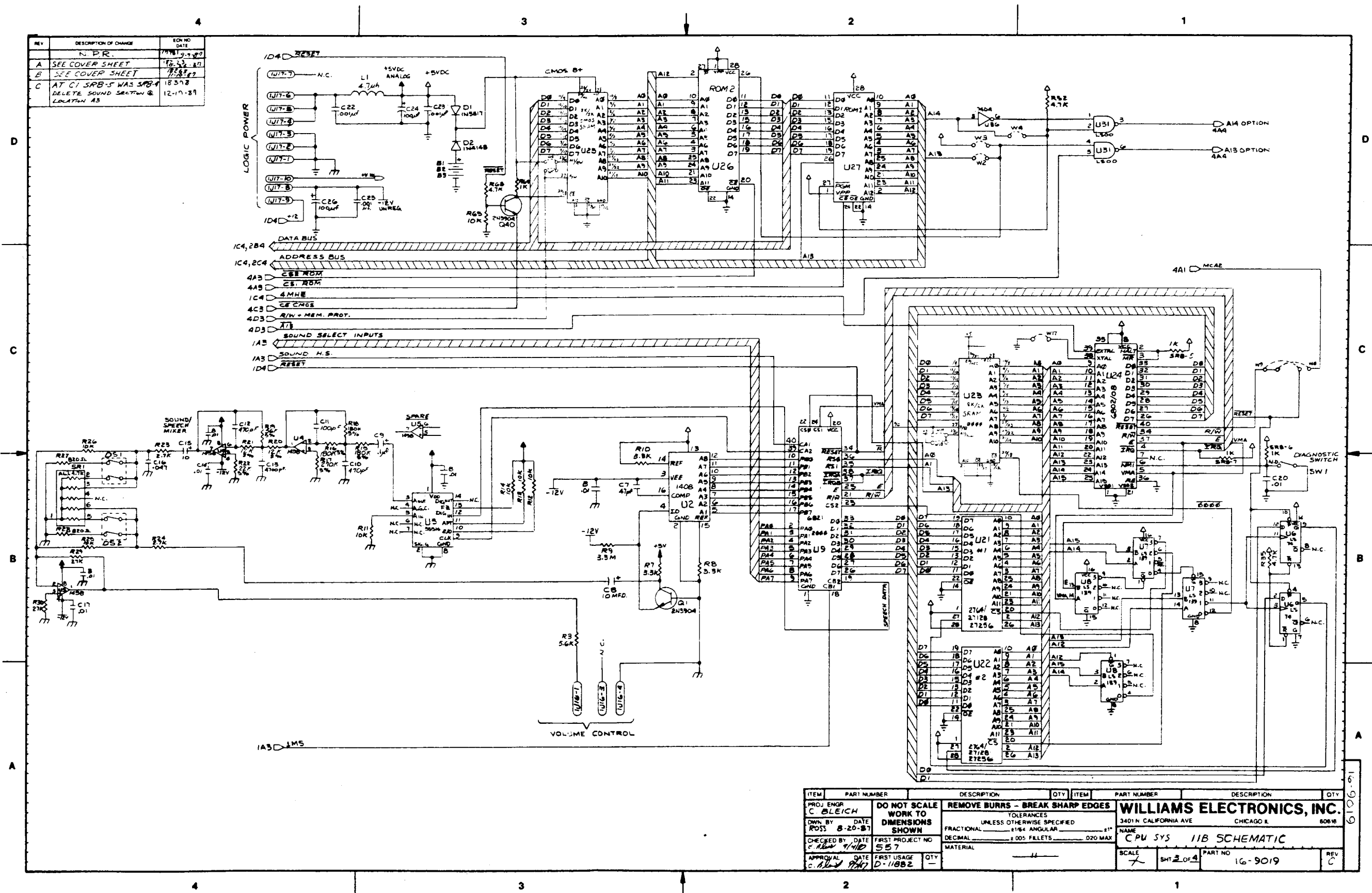
System 11B CPU Schematic (16-9019, Sheet 3 of 4)
