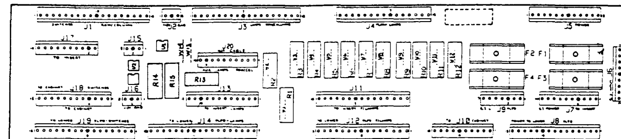
Backbox Interconnect Board p/n D-12313-2011
