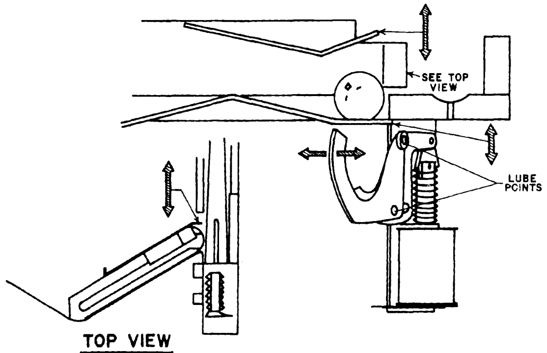
Figure 3. Adjustments and Lubrication Points, Shooter Lane Feeder.
