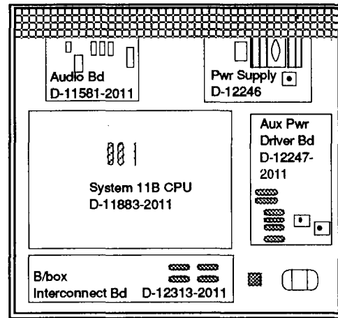
BACKBOX
