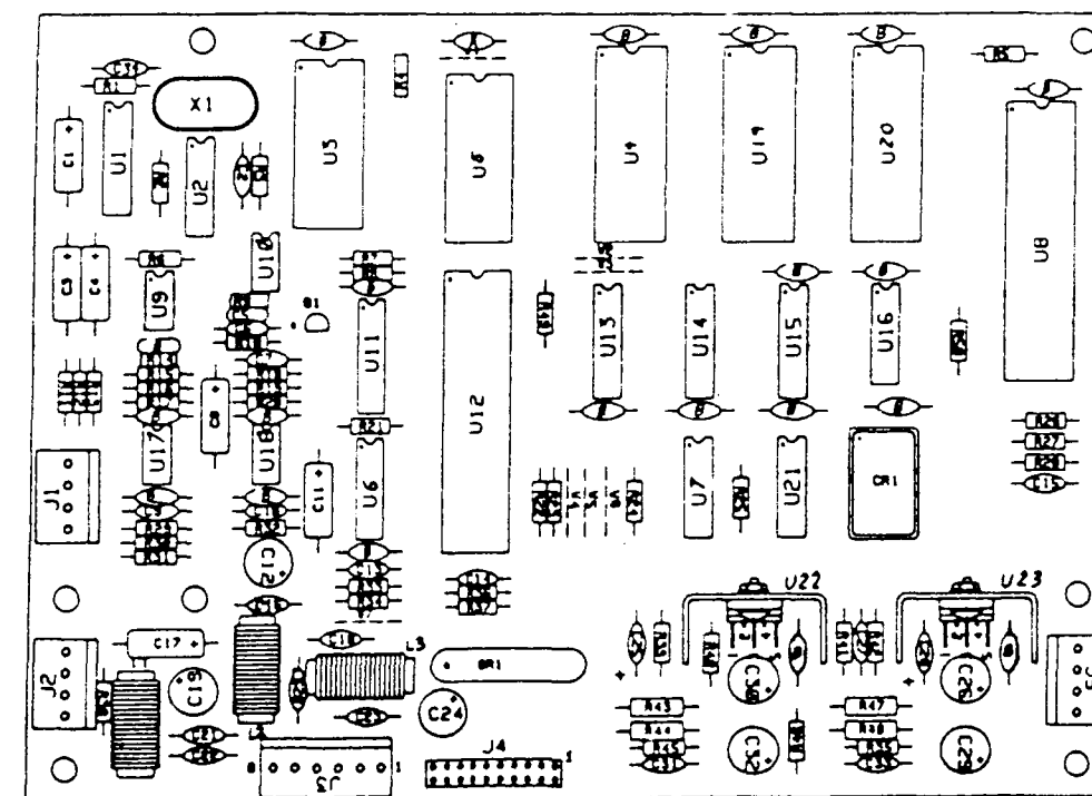
Audio Board Assembly p/n D-11581-2011
