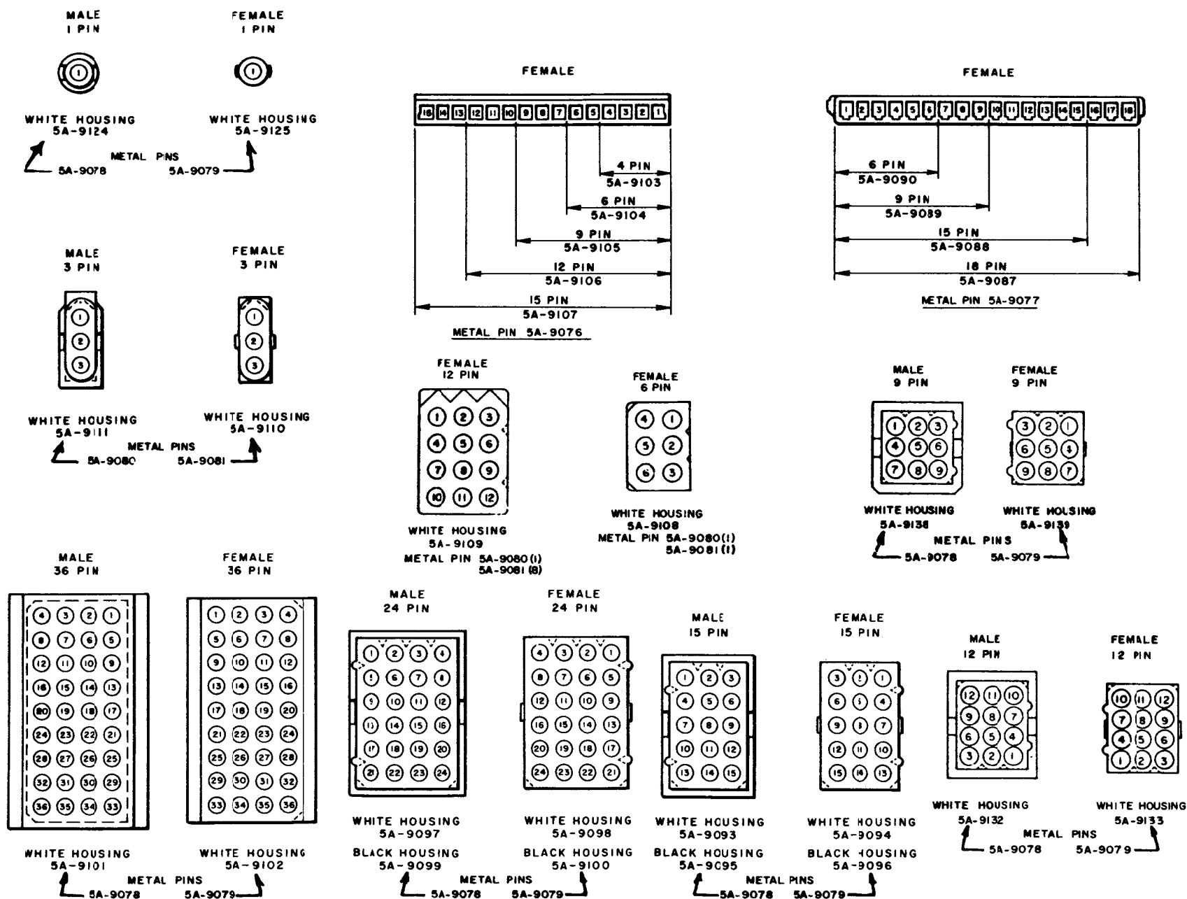
Figure 13. Connector Details
