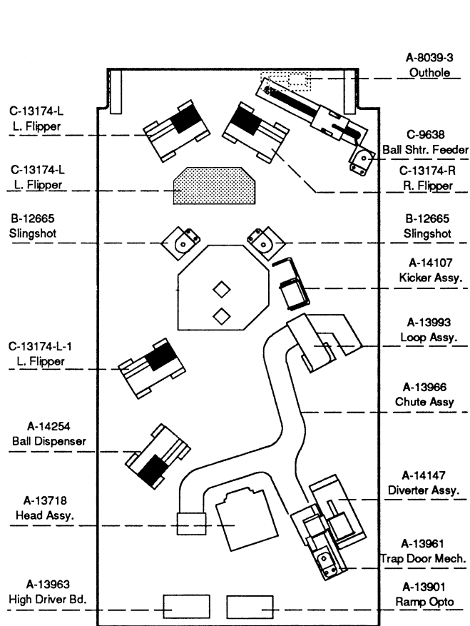
Under Side of Playfield, Viewed in Raised Position
