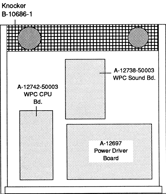
Backbox
