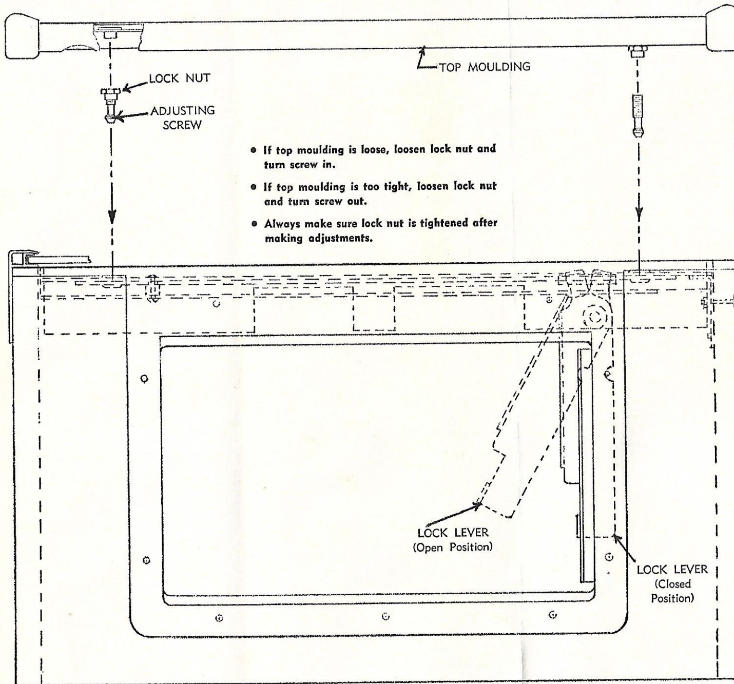
CABINET FRONT
