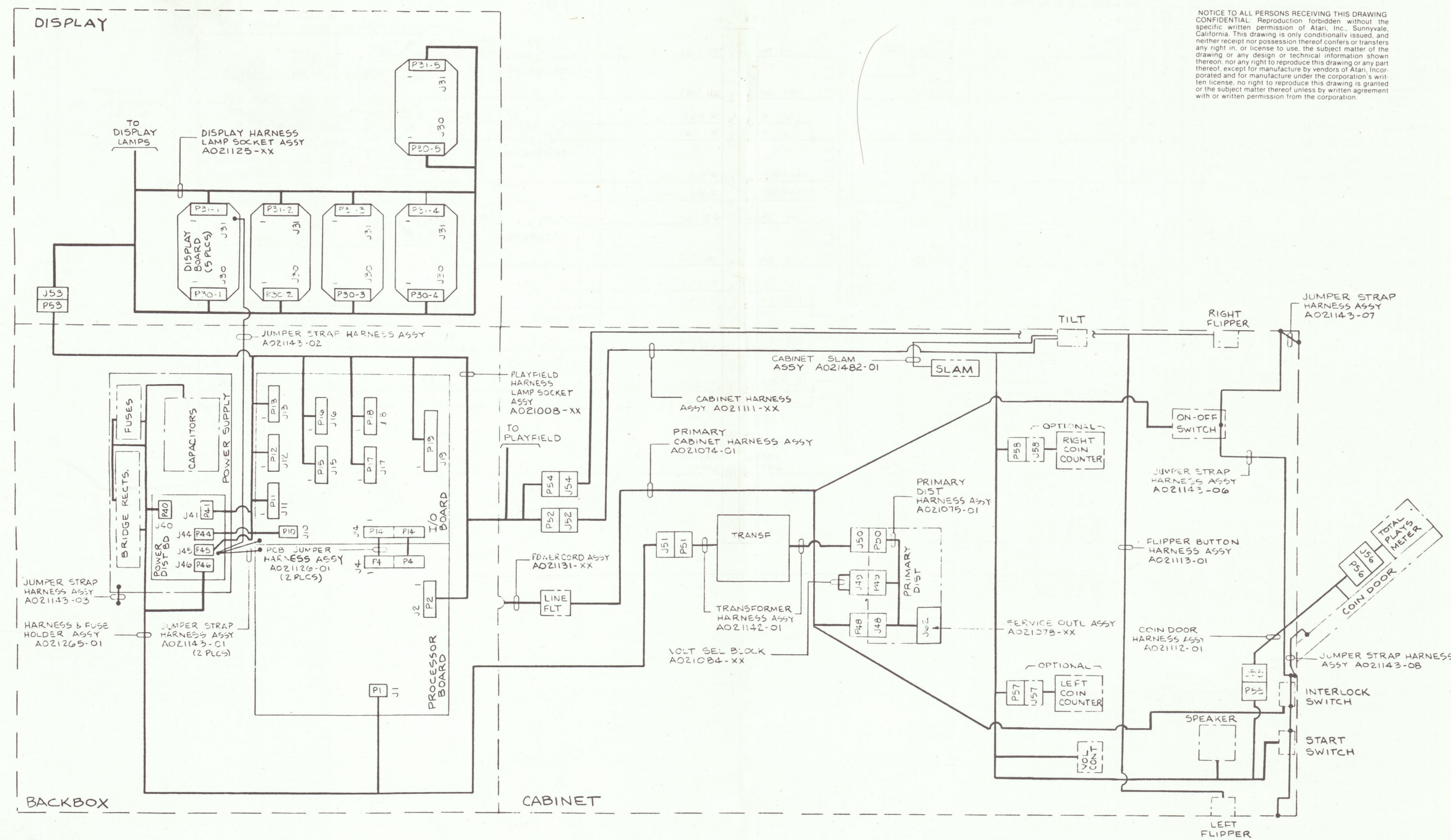
Superman Interconnect Diagram 021278-01 B
