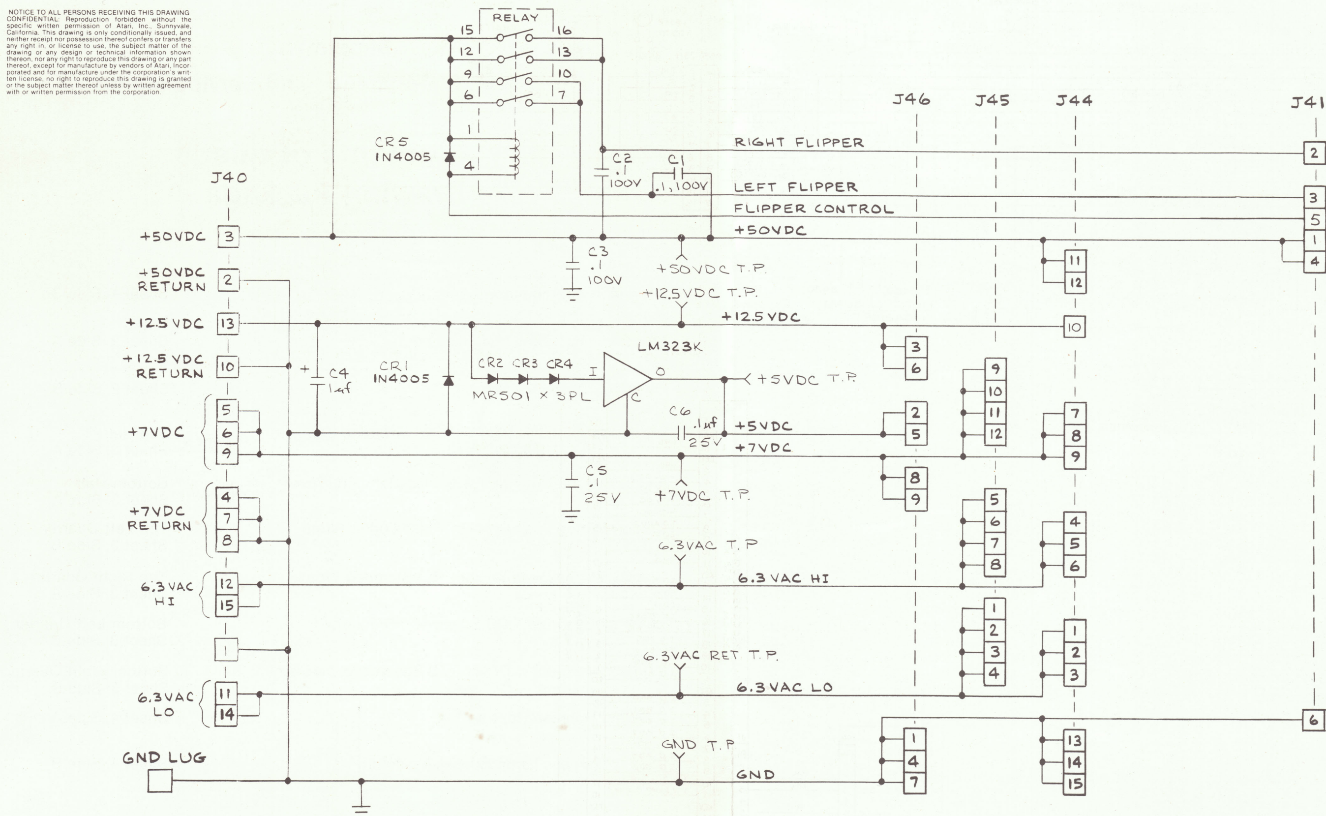
Power Distribution P.C.B. Schematic Diagram 020921-01 B
