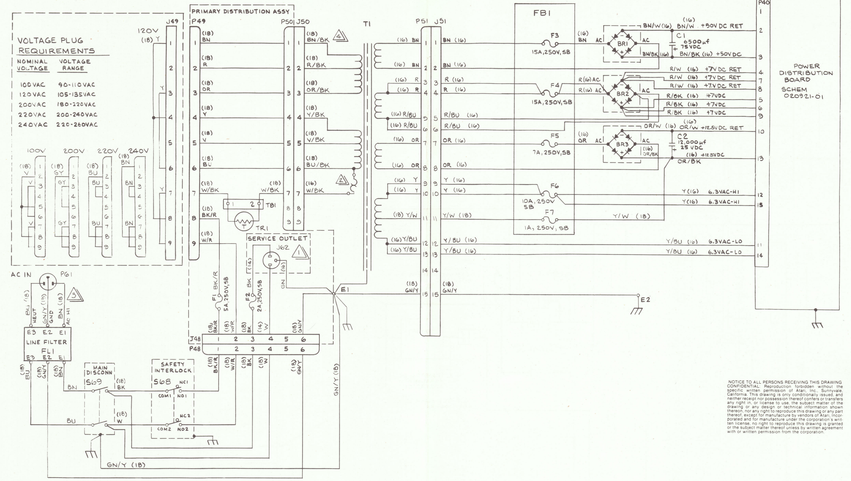
Power Supply Wiring Diagram 021003-01 B
