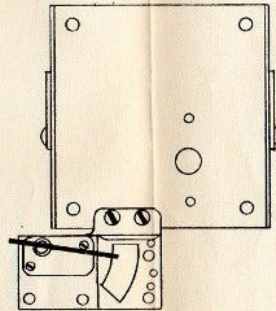
Coin Switch Bracket 25c Play
