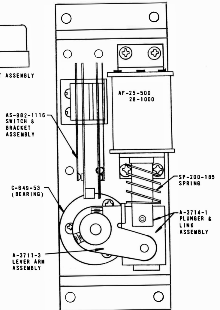
AS-1587-97 FLIPPER UNIT (RIGHT) (AS SHOWN)
