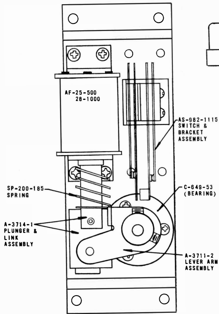
AS-1587-98 FLIPPER UNIT (LEFT) (AS SHOWN)
