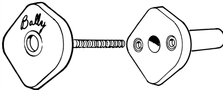
SHOOTER HOUSING COVER PART NO. A-3830
