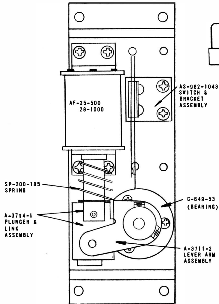
AS-15B7-88 FLIPPER UNIT (LEFT) (AS SHOWN)
