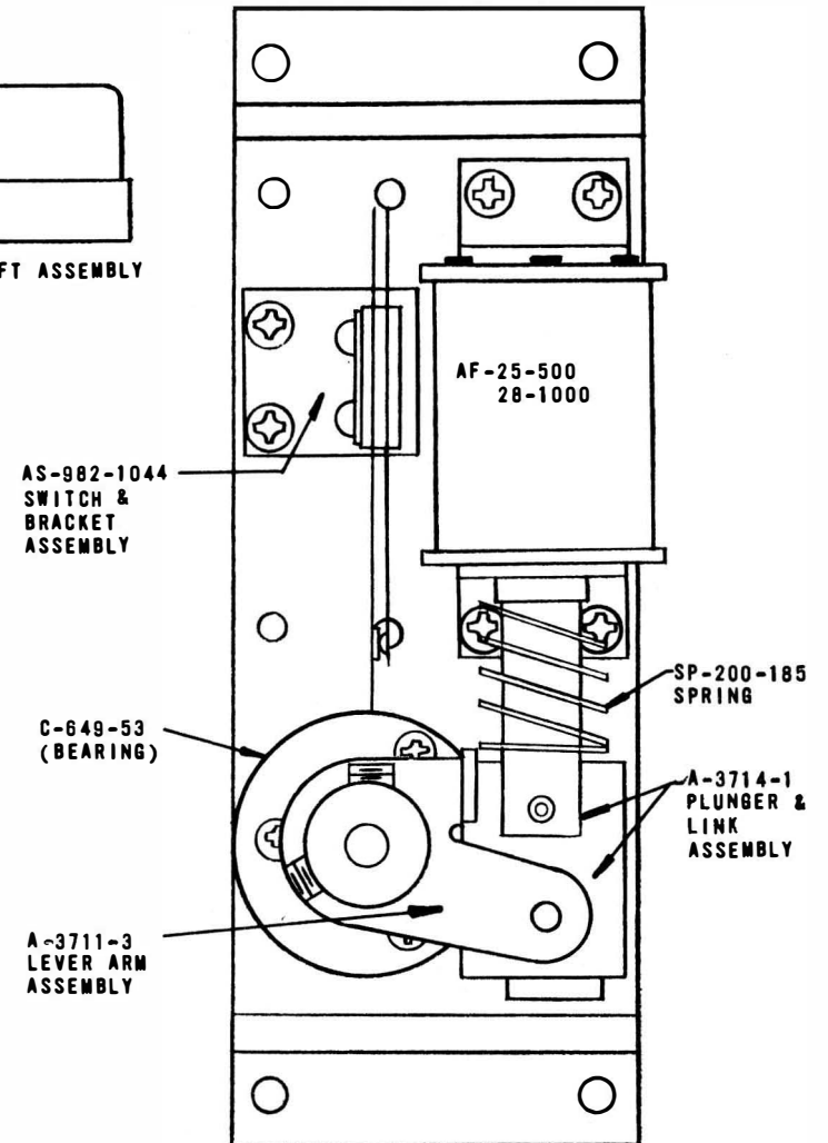
AS-15B7-89 FLIPPER UNIT (RIGHT) (AS SHOWN)
