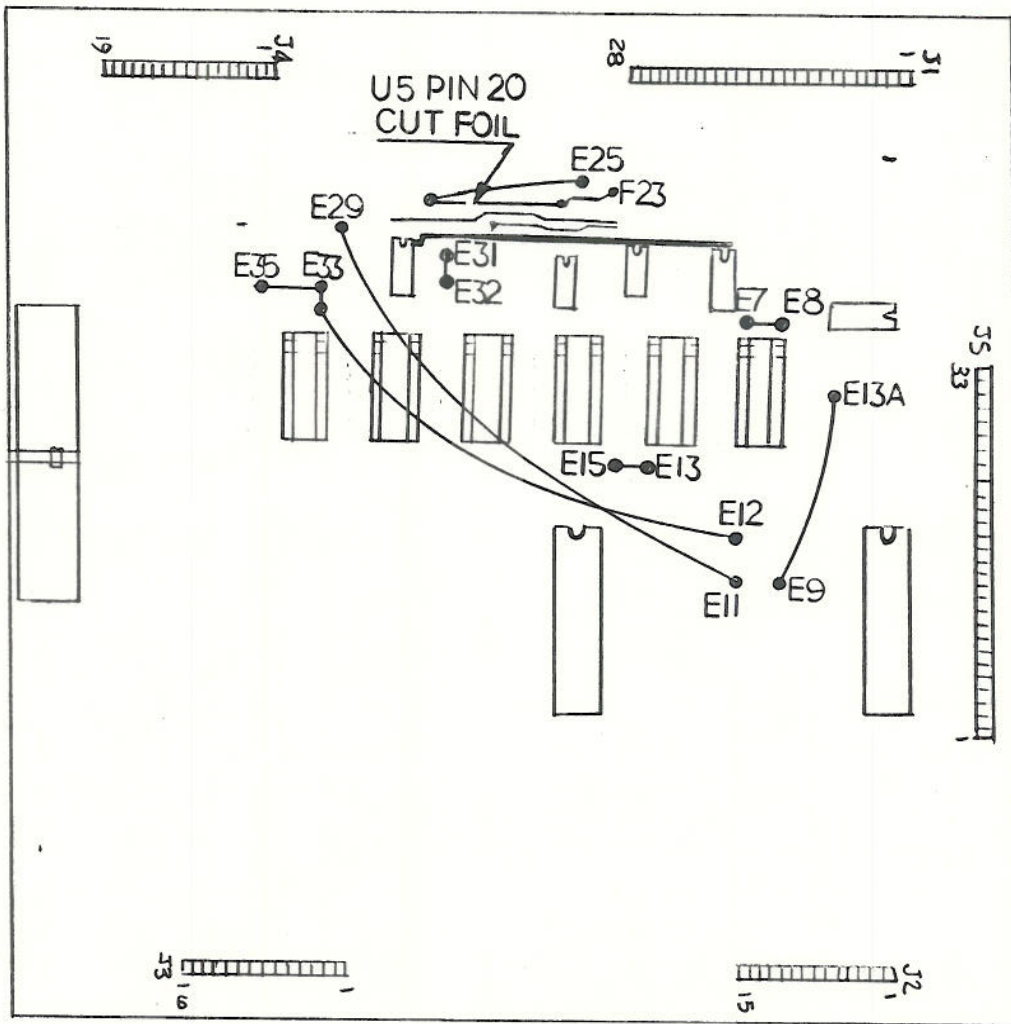
MPU IBOARD AS2518-35
